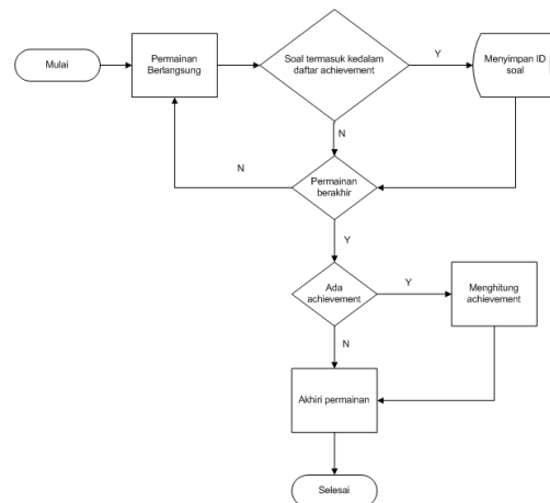
Gambar 3 Flowchart pengecekan achievement
