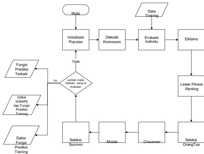
Gambar 3 flowchart proses learning Grammatical Evolution
