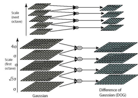
Gambar 2.2 Representasi Difference-of-Gaussian [7]
