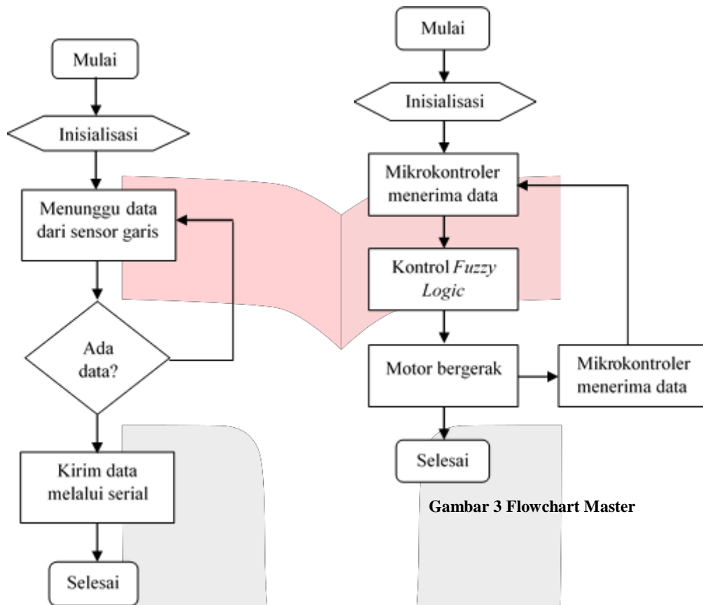
Gambar 2 Flowchart Slave
