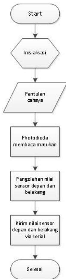
Gambar 4 Flowchart Slave
