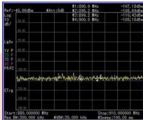
Gambar 11 Scanning Frequensi Speqtrum Analyzer (after)
