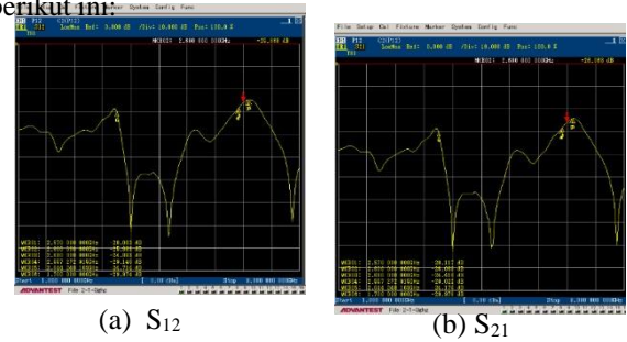
Gambar 4.5 Grafik mutual coupling antenna MIMO metamaterial
