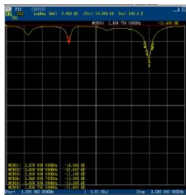
Gambar 4.2 Hasil pengukuran Return Loss (S 22 ) antenna MIMO metamaterial
