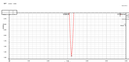
Gambar 3.5 Simulasi VSWR antenna konvensional
