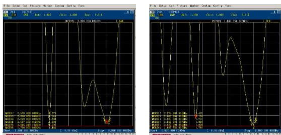
(a) VSWR Port1 (b) VSWR Port 2
