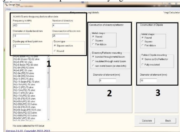
Gambar 3-3 Proses Perhitungan Ukuran Antena
