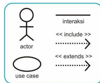
Gambar 2 Simbol Use Case Diagram
