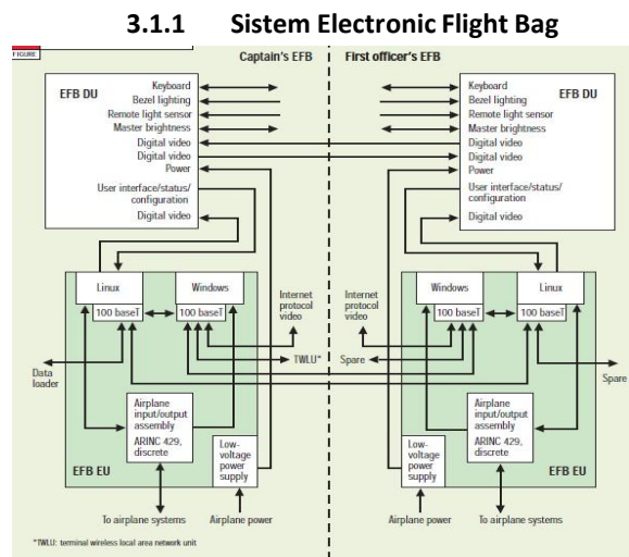
Gambar 3-1 Sistem EFB Asli
