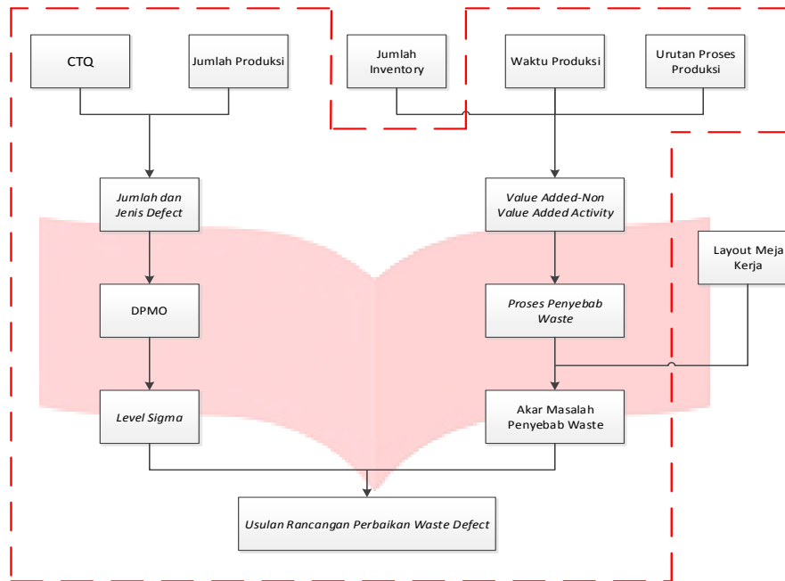
Gambar 1. Model konseptual
