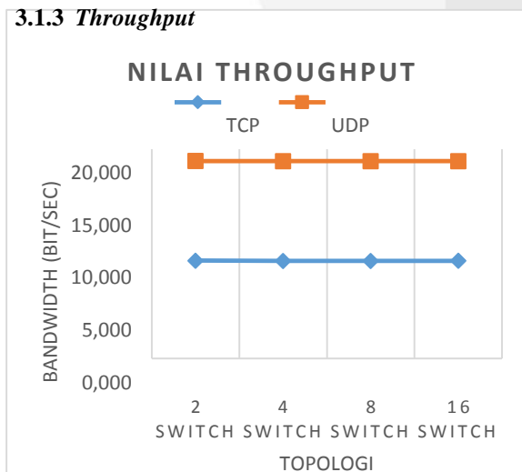
Gambar 3.1.3 Nilai Throughput
