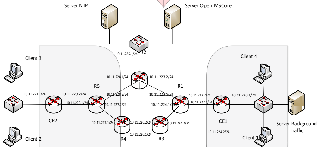
Gambar 3. 1 Topology Sistem
