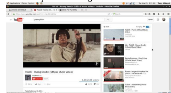
Gambar 4.68 Tampilan Streaming
