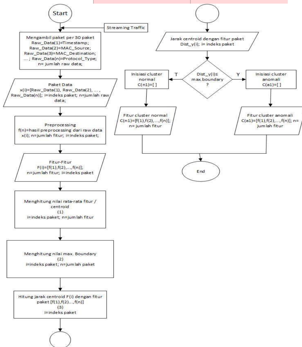
Gambar 3.2 Flowchart Algoritma Clustream (Microclustered)
