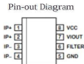
Gambar 5. Sensor Arus
