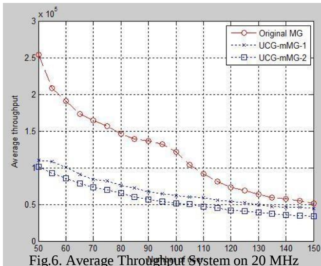
Fig.6. Average Throughput System on 20 MHz Bandwidth
