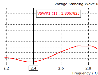
Gambar 3. 3 VSWR 2.4 GHz
