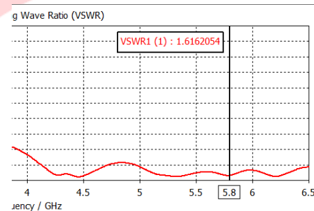
Gambar 3. 11 VSWR 5.8 GHz
