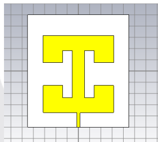
Gambar 3. 1 Antena Double E-Shaped
