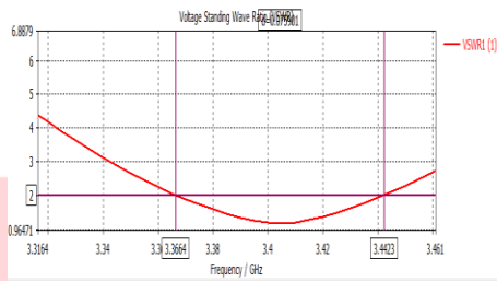
Gambar 3. 8 Bandwidth 3.4 GHz
