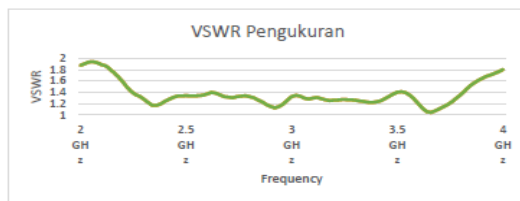
Gambar 4.1 VSWR
