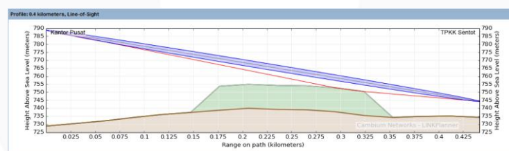
Gambar 4 Perancangan wireless outdoor station TPKK Sentot
