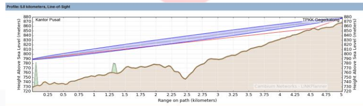
Gambar 3 Perancangan wireless outdoor station TPKK Gegerkalong
