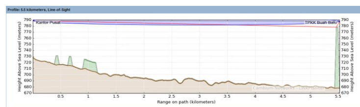
Gambar 5 Perancangan wireless outdoor station TPKK Buah Batu
