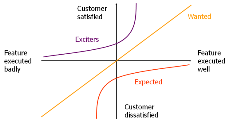
Gambar 4 Model Kano
