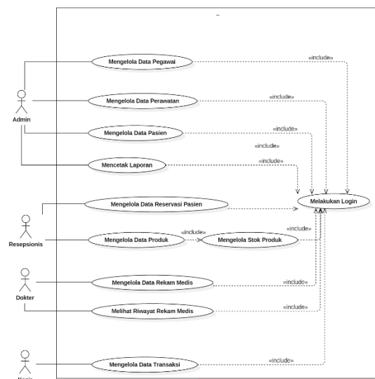
Gambar 3.9 Usecase Diagram
