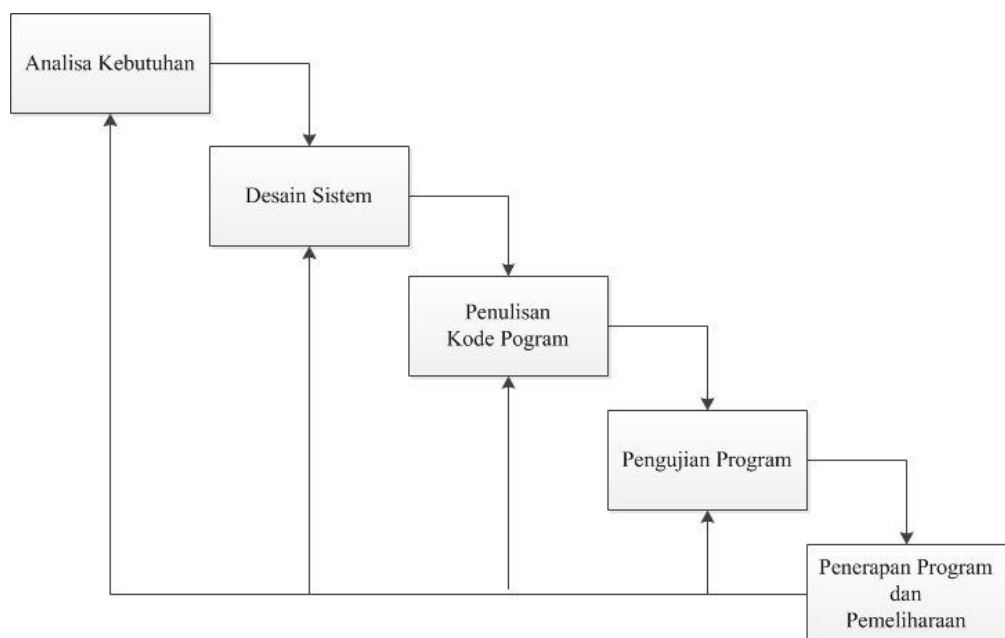
Gambar 1.1 Metode waterfall
