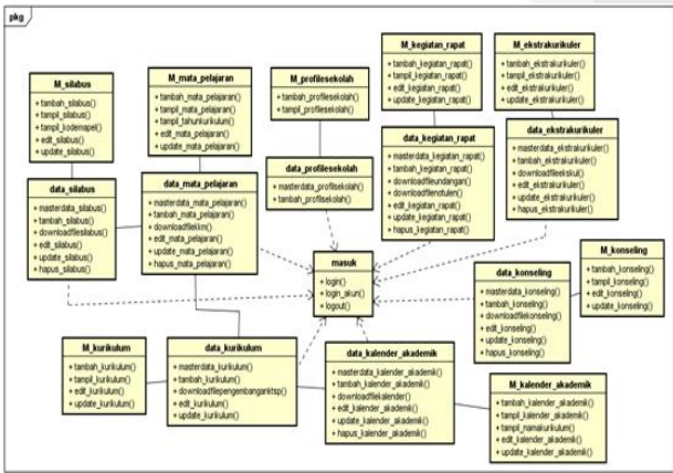
Gambar 3.4 Class Diagram
