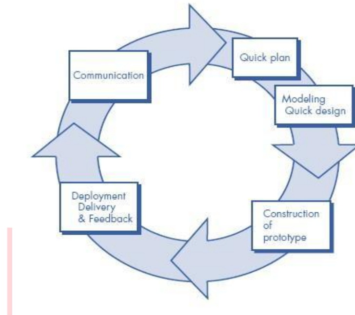
Gambar 1 Metode Prototype
