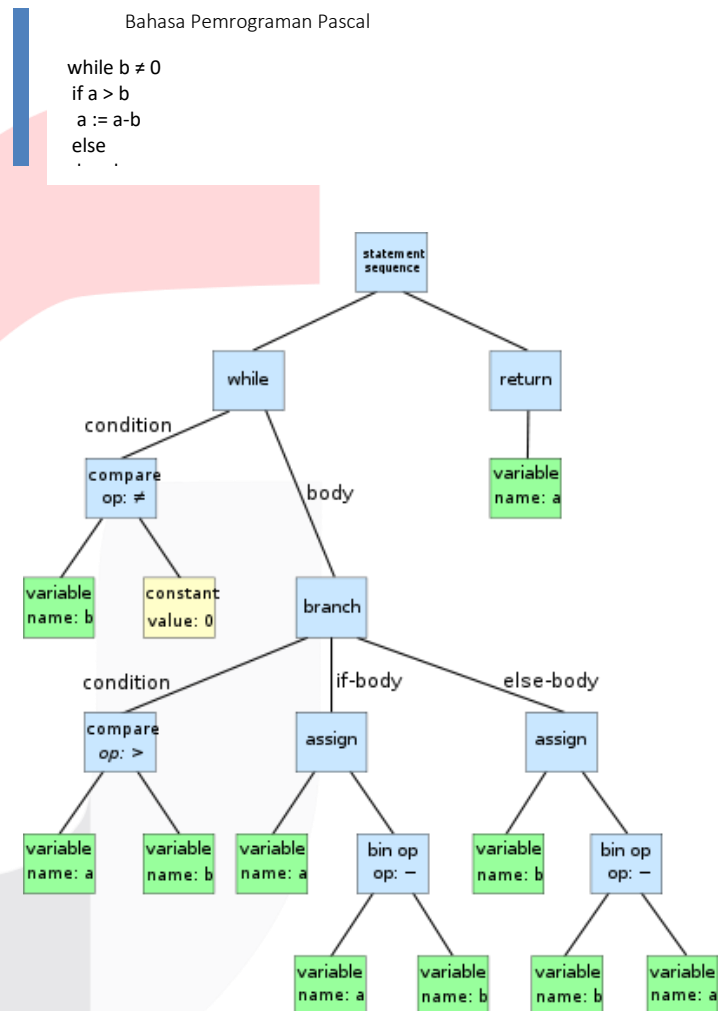
Gambar 2-1 Abstract Syntax Tree
