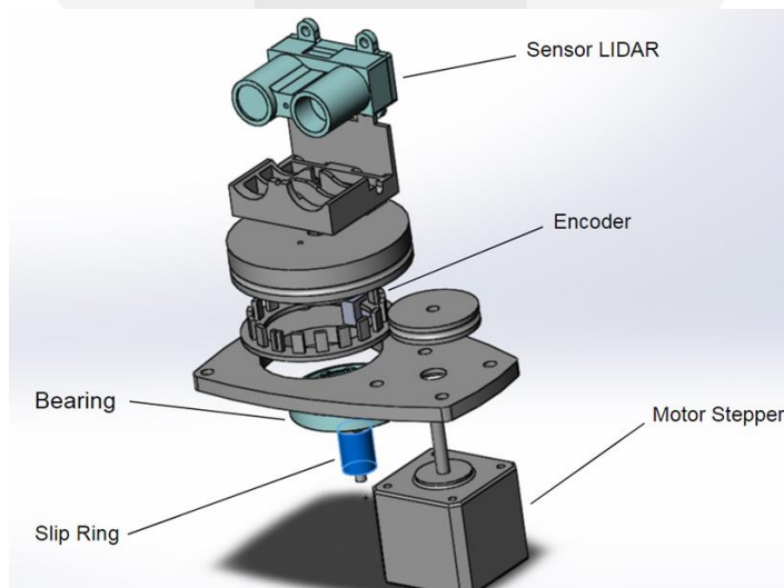
Gambar 3. Rancangan Hardware
