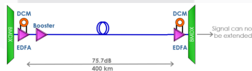
Gambar 2.4 Repeater-less
