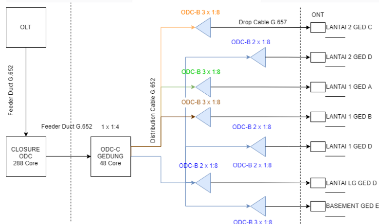
Gambar 3.3 Topologi FTTB Mall Cihampelas Walk
