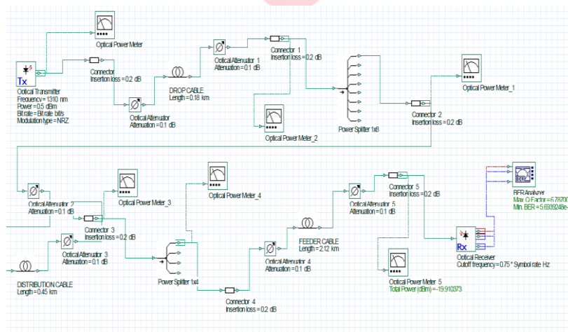
Gambar 3.5 Simulasi Jaringan arah upstream
