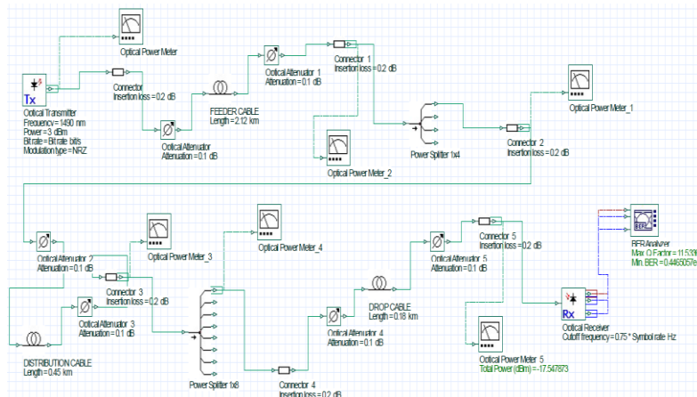
Gambar 3.4 Simulasi Jaringan arah downstream
