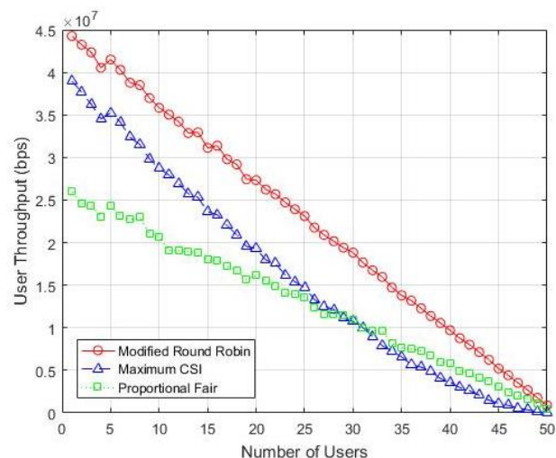
Figure 6. User Throughput
