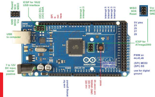
Gambar 2.5 Arduino Mega 2560
