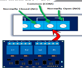
Gambar 2.6 Relay 4 Channels
