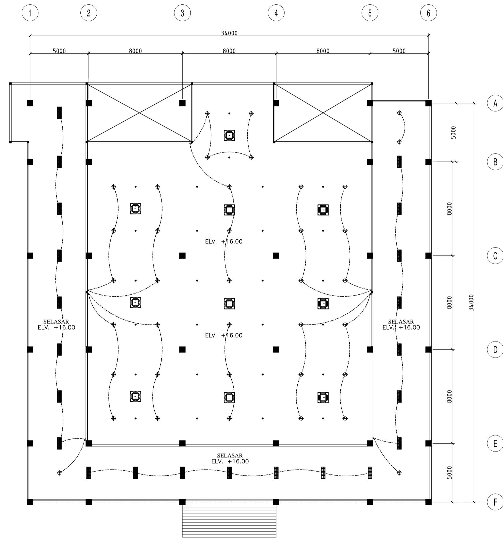
DENAH CEILING LANTAI 2 (MASJID) SCALE 1:150
