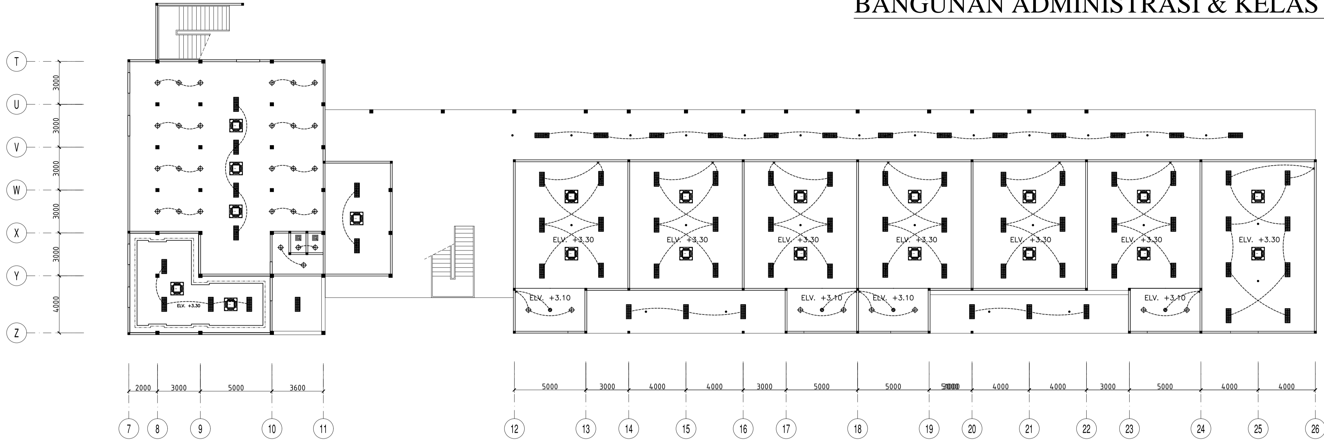
DENAH CEILING LANTAI DASAR SCALE 1 : 450
