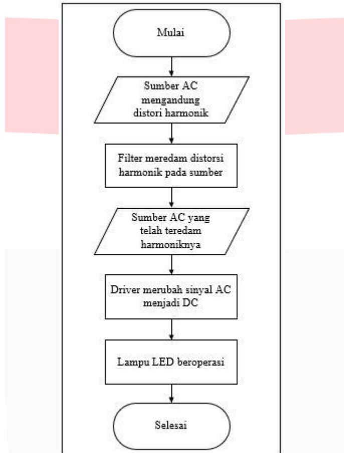
Gambar 3.3. Proses Kerja Driver Lampu LED dan Filter
