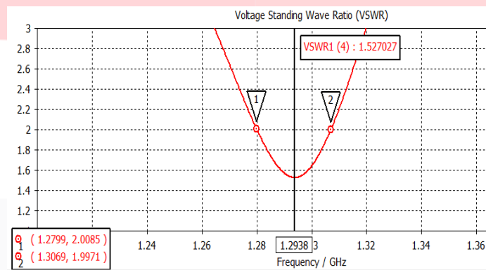
Gambar 5. Nilai Bandwidth
