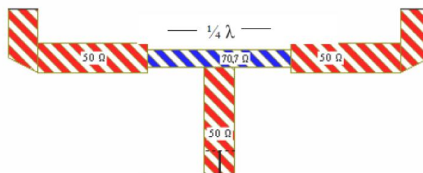
Gambar 3.2 Model T-Junction
