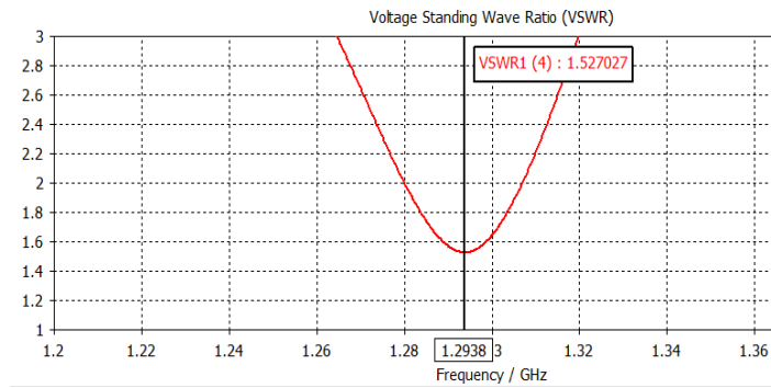
Gambar 4. Nilai VSWR
