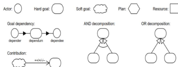
Gambar 1. Metamodel Tropos [1].
