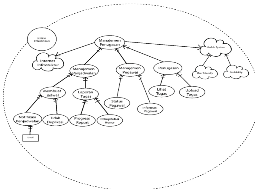
Gambar 5. Model Goal Late Requirement.
