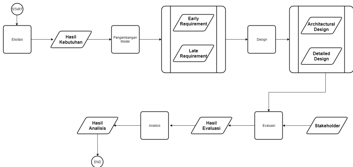
Gambar 2. Alur Penelitian
