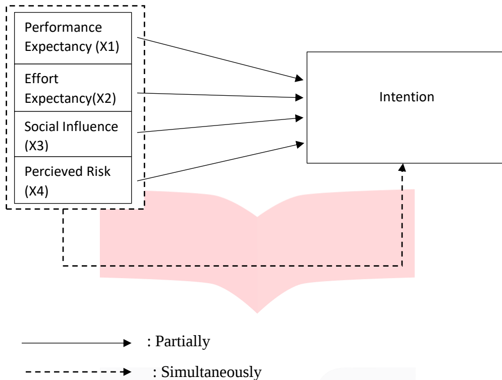
Figure 2.2 Conceptual Framework
