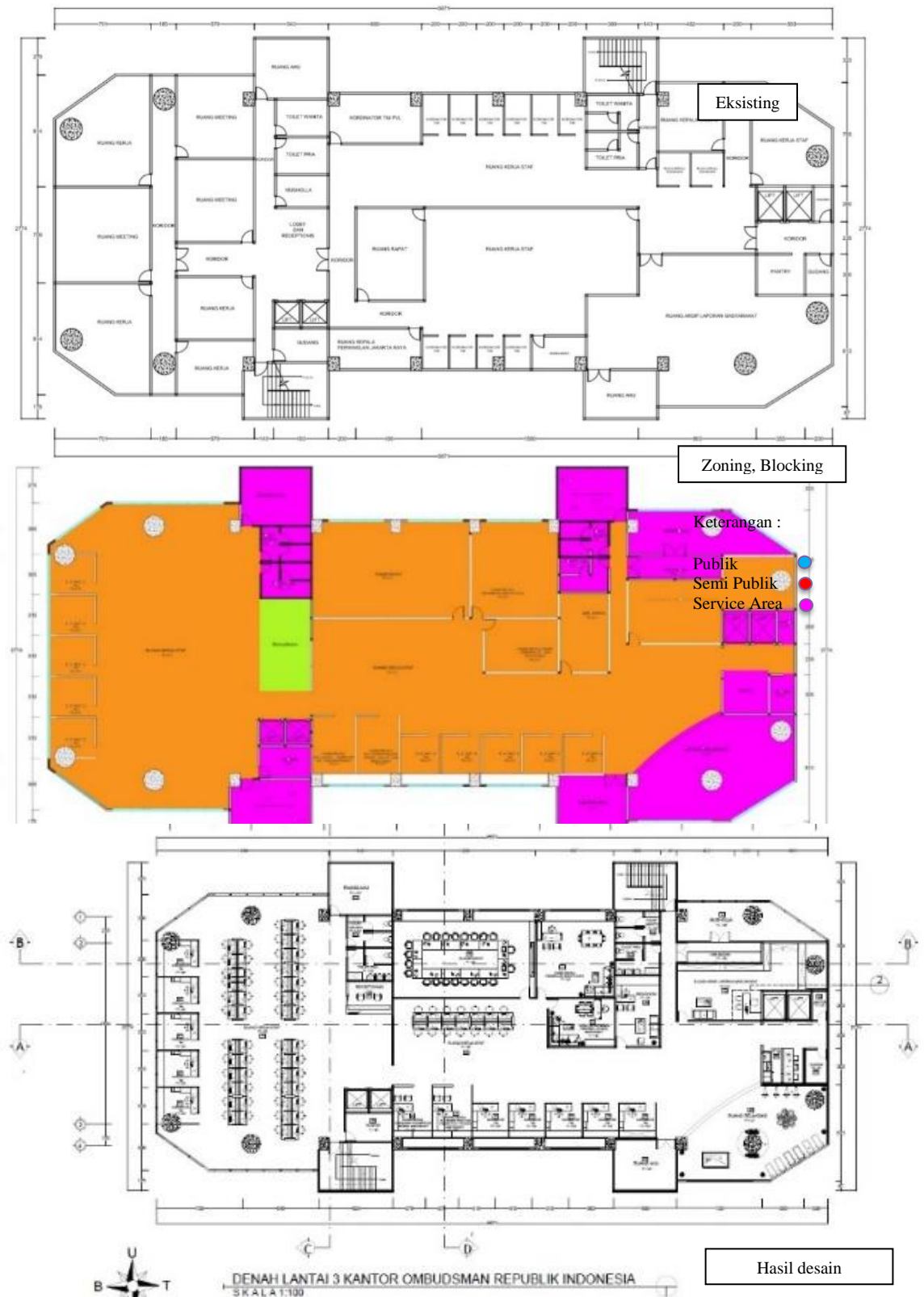
Gambar 4.2 Layout Lantai 3
