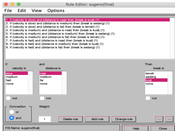
Gambar 3.6: Fuzzy rule.
