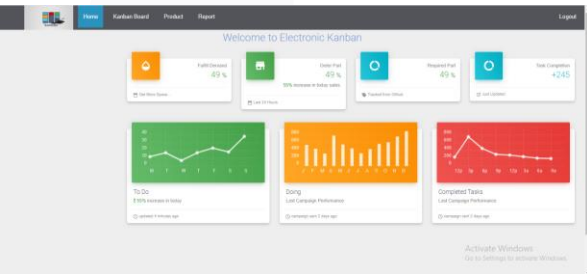
Figure.6 Dashboard Interface
