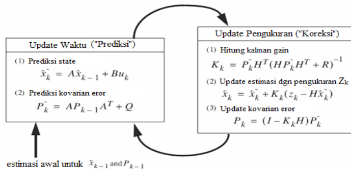
Gambar 2. Proses Kalman Filter
