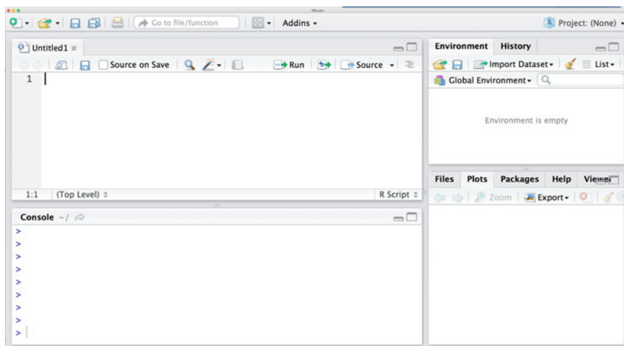
Fig. 28.1 RStudio interface
