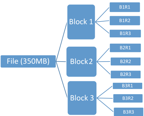
Fig. 4.5 Hadoop architecture (inspired from Hadoop architecture available on https://technocents.files.wordpress.com/2014/04/hdfs-architecture.png (accessed on Aug 10, 2018))
