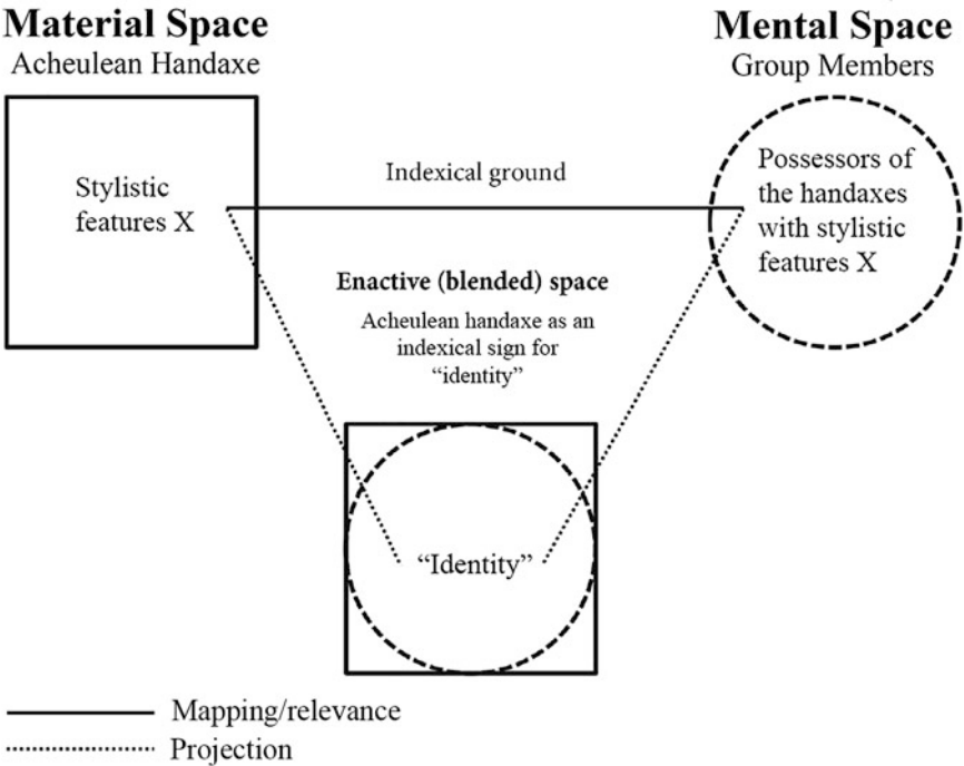
Fig. 19.2 Diagram of the blending process for the concept of identity from the indexical ground created by the recurring association of handaxes’ stylistic features and the presence of the same individuals (group members). The stylistic features X of a local tradition of handaxes occupy the material space (above, left). A viewer understands that the handaxes are owned by the members of a certain group, and this happens within her mental space (above, right). The physical contiguity between the X-shaped handaxes and the presence of some group members embodies the indexical ground. A concept of identity allegedly emerges out of the blending of the two aforementioned elements. Redrawn from Iliopoulos (2016a)
