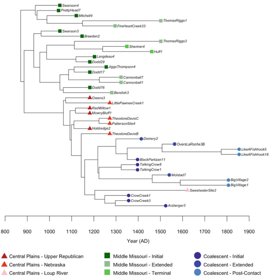
Fig. 9.4 Time-calibrated maximum clade credibility tree
