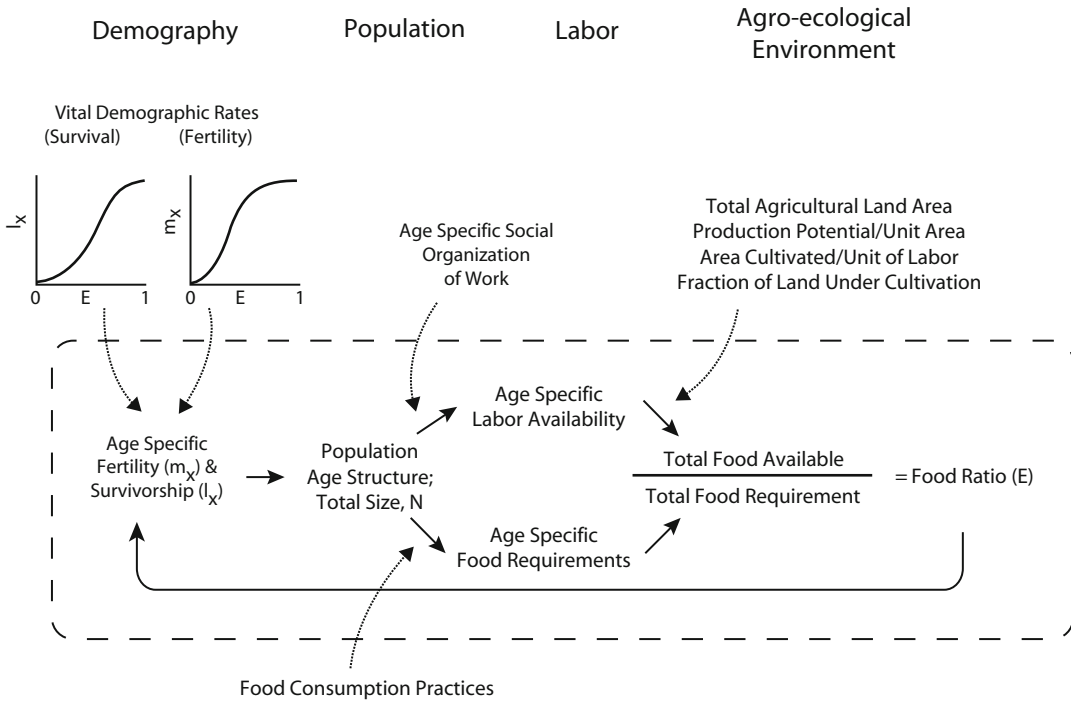
Fig. 16.1 The space-limited population ecology model. Core components of the model and their causal connections (solid arrows) are shown within the dashed line rectangle. Demographic, biosocial, and agroecological factors determining the form and parameter values assigned to those core components are shown around the circumference, with dotted arrows indicating their point of action. We provide a step-by-step description of one iteration through the core components in the text; a more complete description of the mathematical and programming details can be found in Puleston et al. (2014) and references therein
