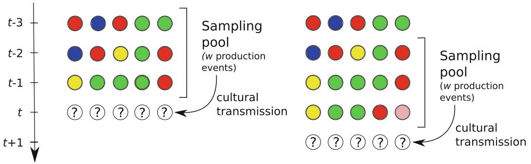
Fig. 5.6 Scheme of the transmission dynamic. In each production event v instances of cultural variants are produced and the probability with which one of the existing variants is produced is given by Eq. (5.13). For instance, in the left figure any of the five instances at time t turns red with probability \frac{(5/15)^{1-b}}{(5/15)^{1-b} + (2/15)^{1-b} + (6/15)^{1-b} + (2/15)^{1-b}} (1 - \mu) . With probability \mu an entirely new variant is introduced (see the pink variant at time t + 1 in the right figure)
