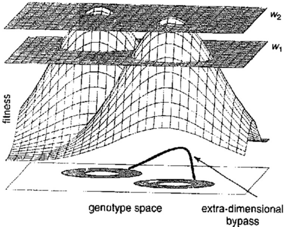
Fig. 7.5 The relationship between a rugged adaptive landscape and a holey adaptive landscape (Gavrilets 1997, p. 311)
