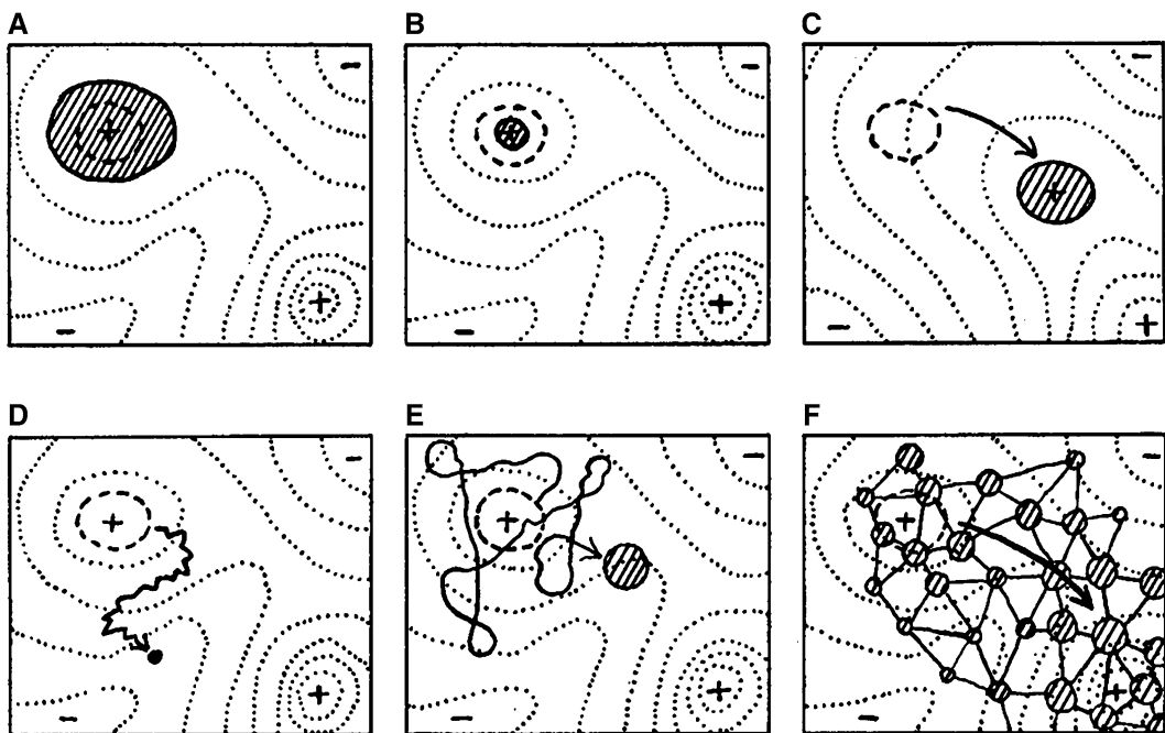
Fig. 7.3 Wright's (1932) diagrams showing gene combinations occupied by a population under various evolutionary scenarios. (a) Increased mutation or reduced selection 4NU , 4NS very large. (b) Increased selection or reduced mutation 4NU , 4NS very large. (c) Quantitative change of environment 4NU , 4NS very large. (d) Close inbreeding 4NU , 4NS very small. (e) Slight inbreeding 4NU , 4NS medium. (f) Division into local races 4nm medium
