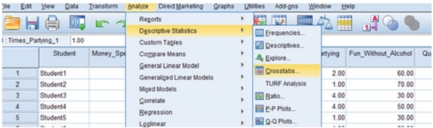
Fig. 7.27 Doing crosstabs in SPSS (first step)
