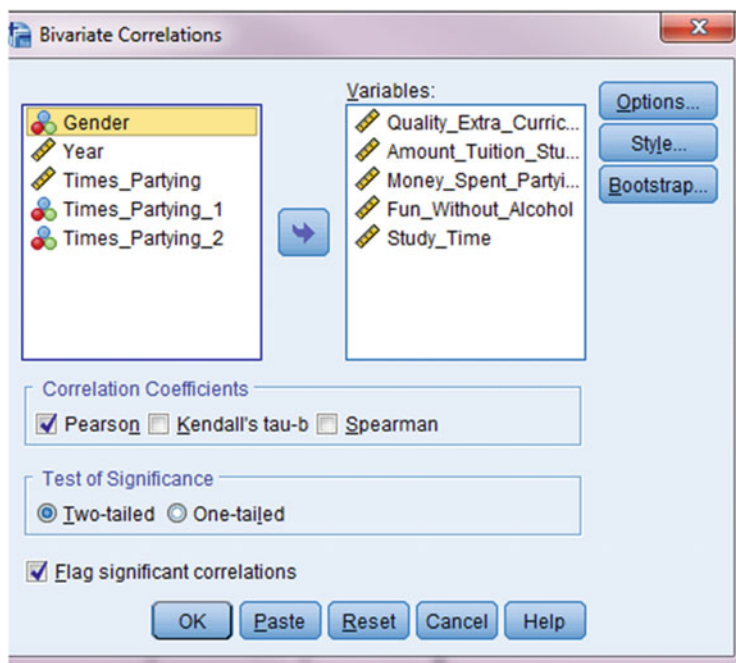
Fig. 8.17 Doing a correlation in SPSS (second step)
