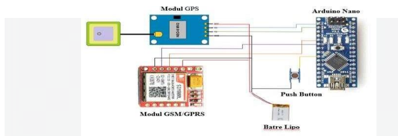
Gambar 2 Skematik Hardware
