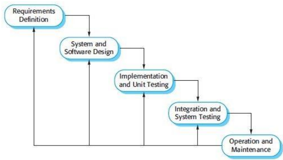
Gambar 1- 1 Model Waterfall [1]
