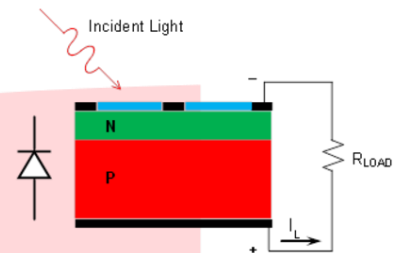
Gambar 2.3 Photovoltaic Device
