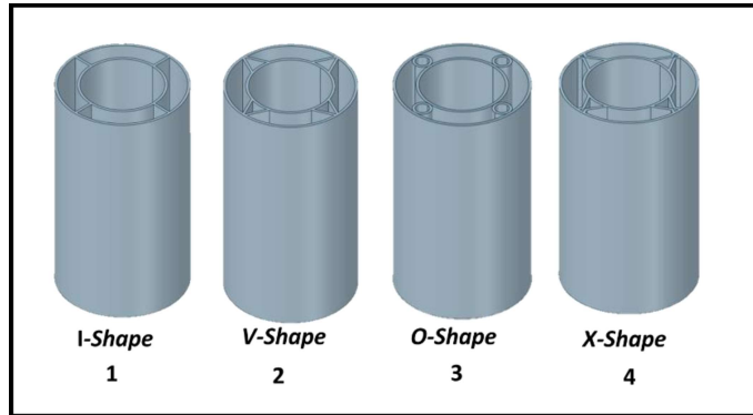
Gambar 4 Struktur Bionic Bamboo Tube
