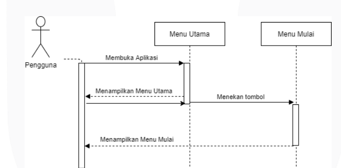
Gambar 3.18 Sequence Diagram Mulai
