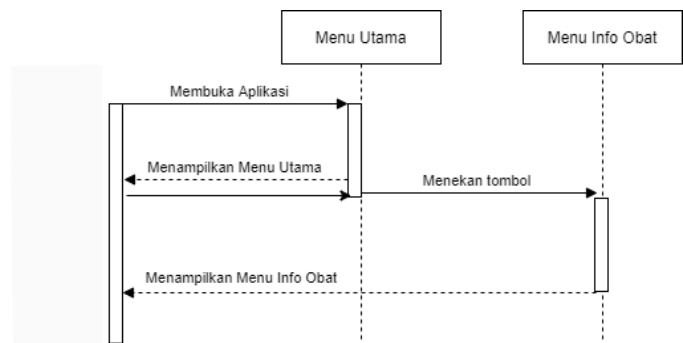
Gambar 3.21 Sequence Diagram Menu Info Obat
