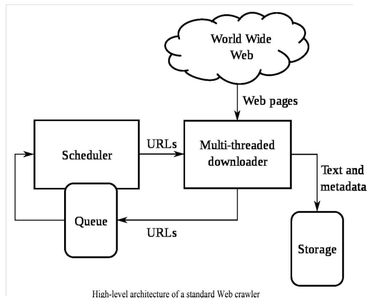
High-level architecture of a standard Web crawler
