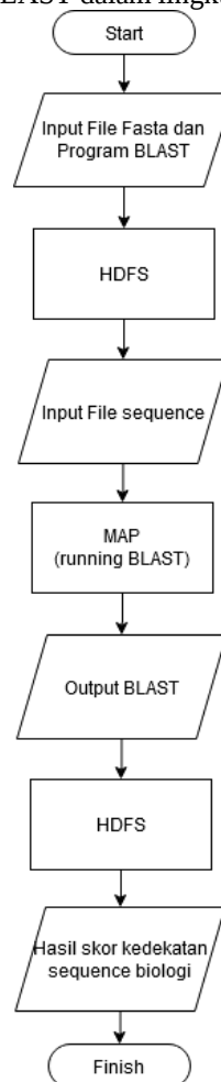
Gambar 9 Flowchart Sistem
